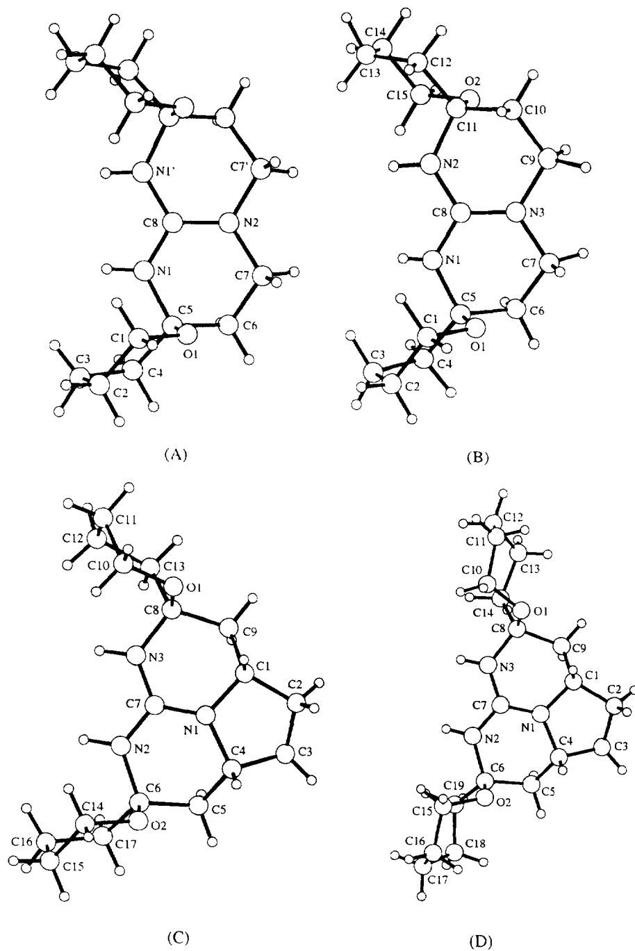
Fig. 3. Structures of the cations [C_{15}H_{26}N_3O_2]^+ in 14 (A) and 15 (B), [C_{17}H_{28}N_3O_2]^+ in 26 (C) and [C_{19}H_{32}N_3O_2]^+ in 30 (D)
